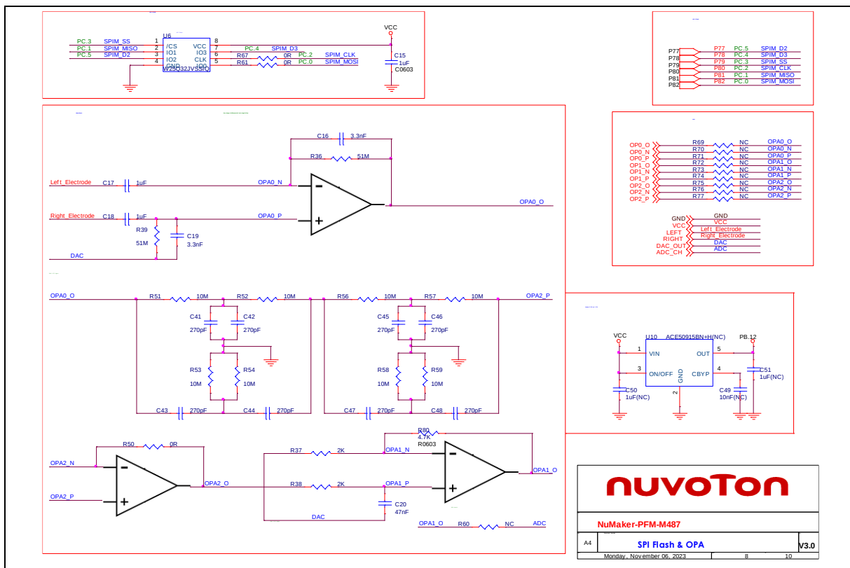
Figure 2-20 Heartbeat Sensor and SPI Flash Circuit
