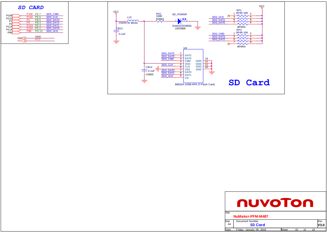
Figure 2-16 MicroSD Card Circuit
