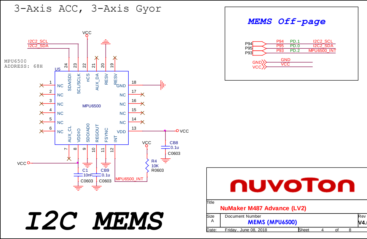
Figure 3-8 I 2 C MEMS Circuit
