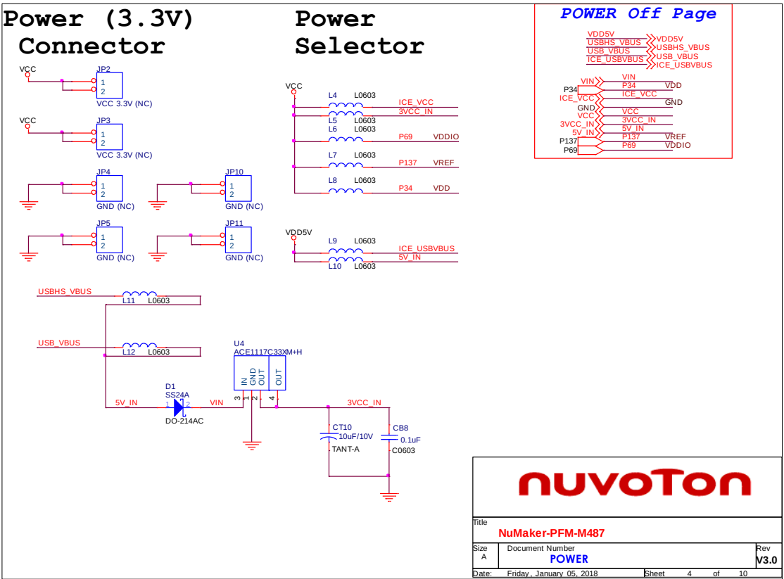
Figure 2-10 Power Circuit and Configurations
