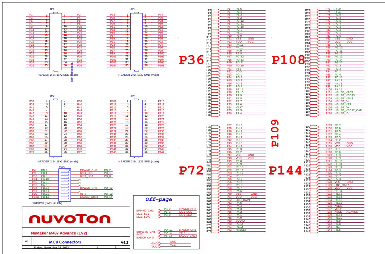
Figure 3-5 Header Connectors
