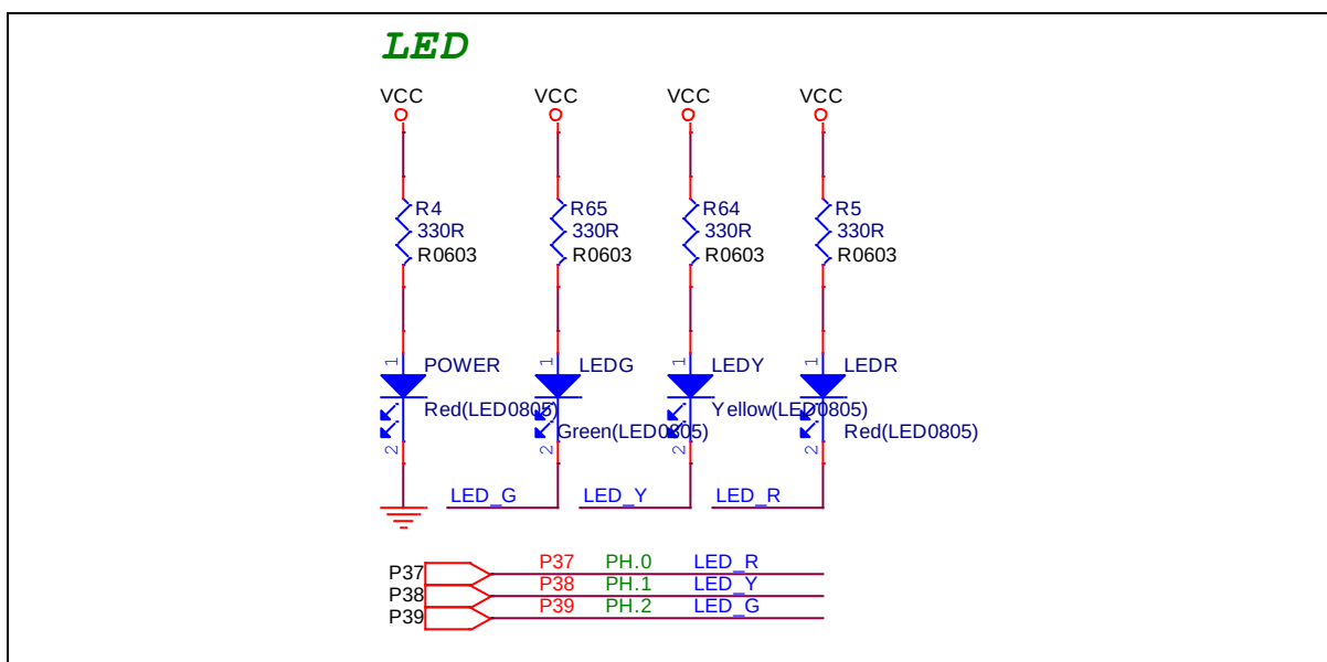
Figure 2-14 Power LED and IO LED Circuit
