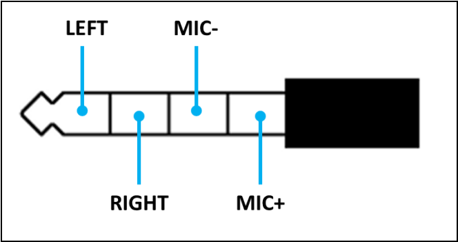
Figure 2-6 3.5mm Phone Jack Diagram
