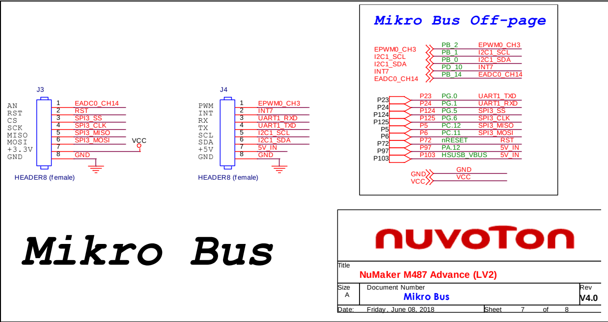
Figure 3-10 Mikro Bus Circuit
