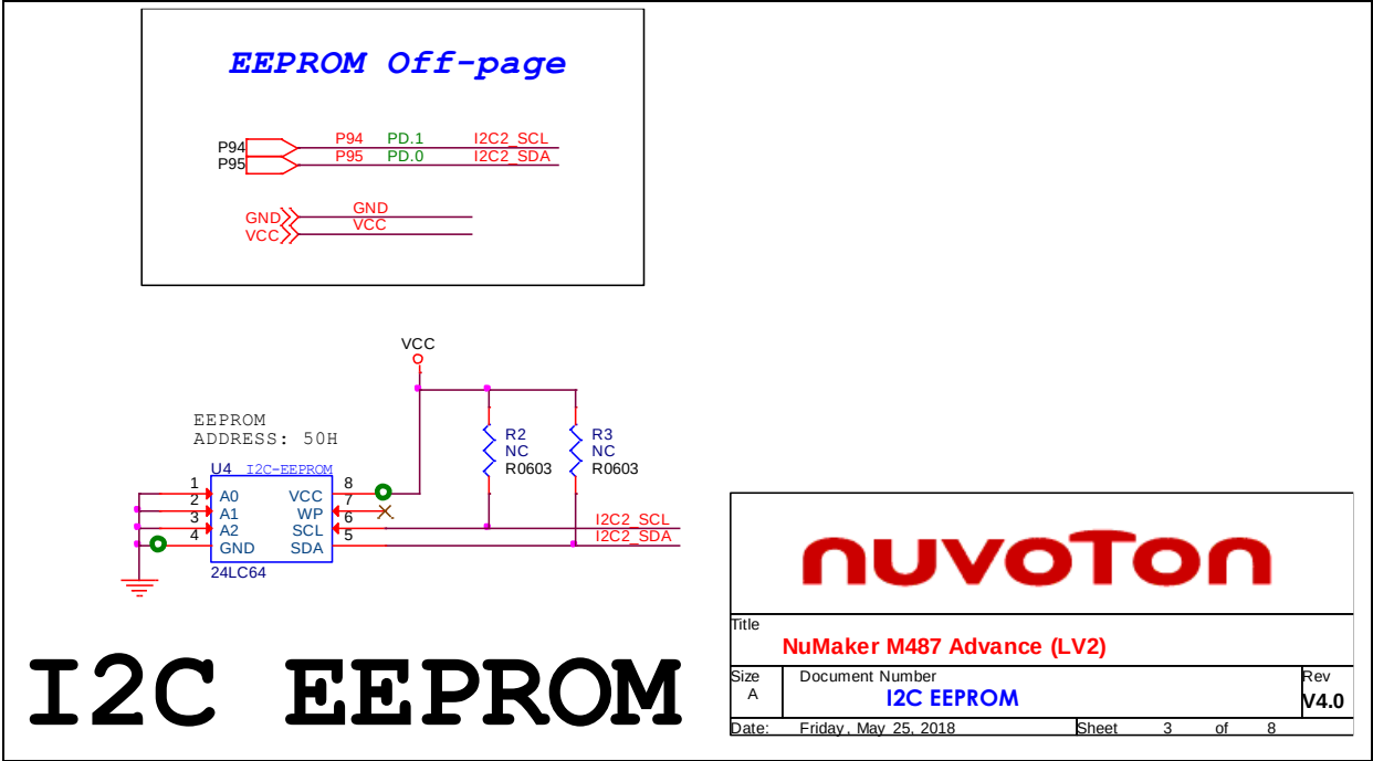
Figure 3-7 I 2 C EEPROM Circuit
