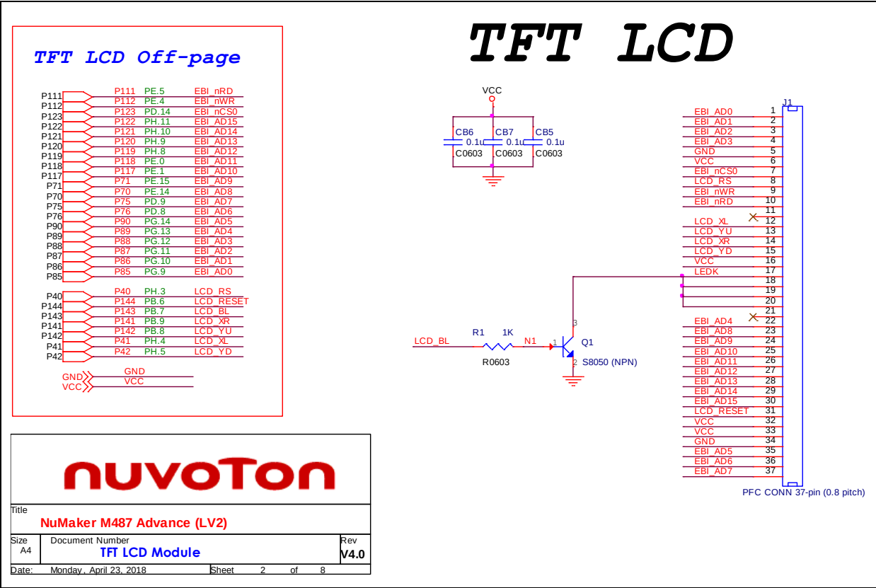
Figure 3-6 QVGA TFT LCD Module with Touch Circuit
