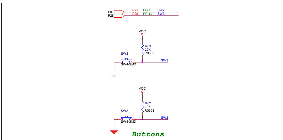
Figure 2-15 Push-Buttons Circuit
