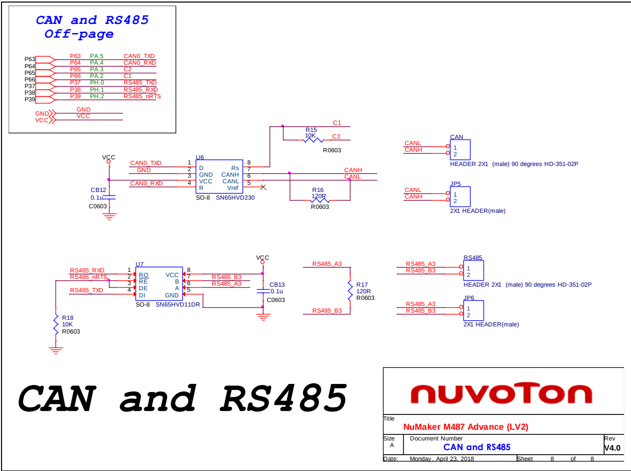
Figure 3-11 CAN and RS485 Circuit
