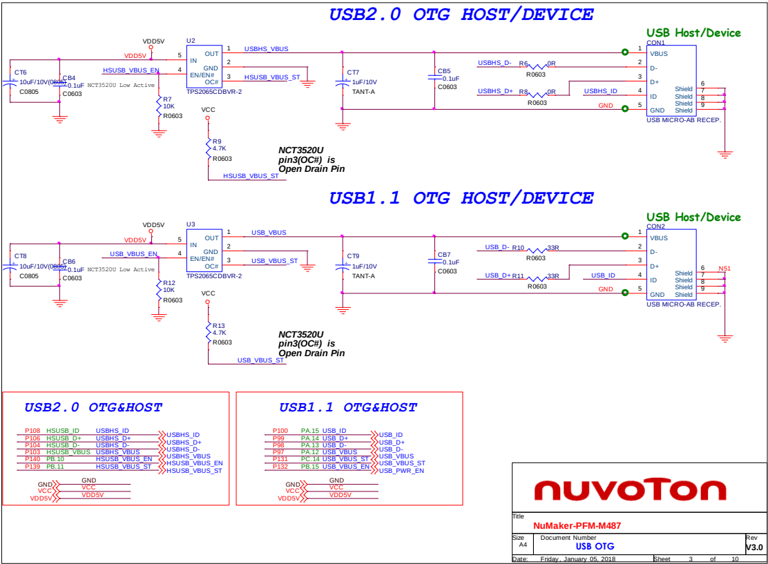
Figure 2-17 USB HS OTG and FS OTG Circuit
