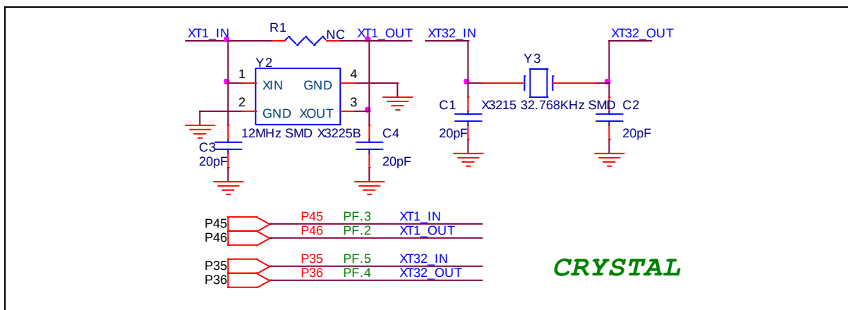
Figure 2-13 External Crystal Circuit
