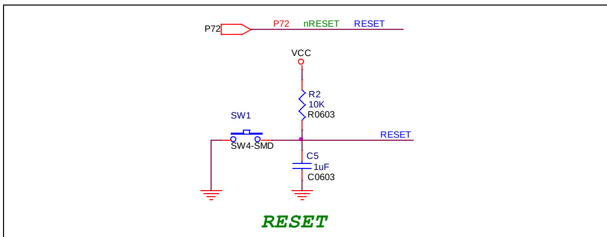
Figure 2-12 Reset Circuit
