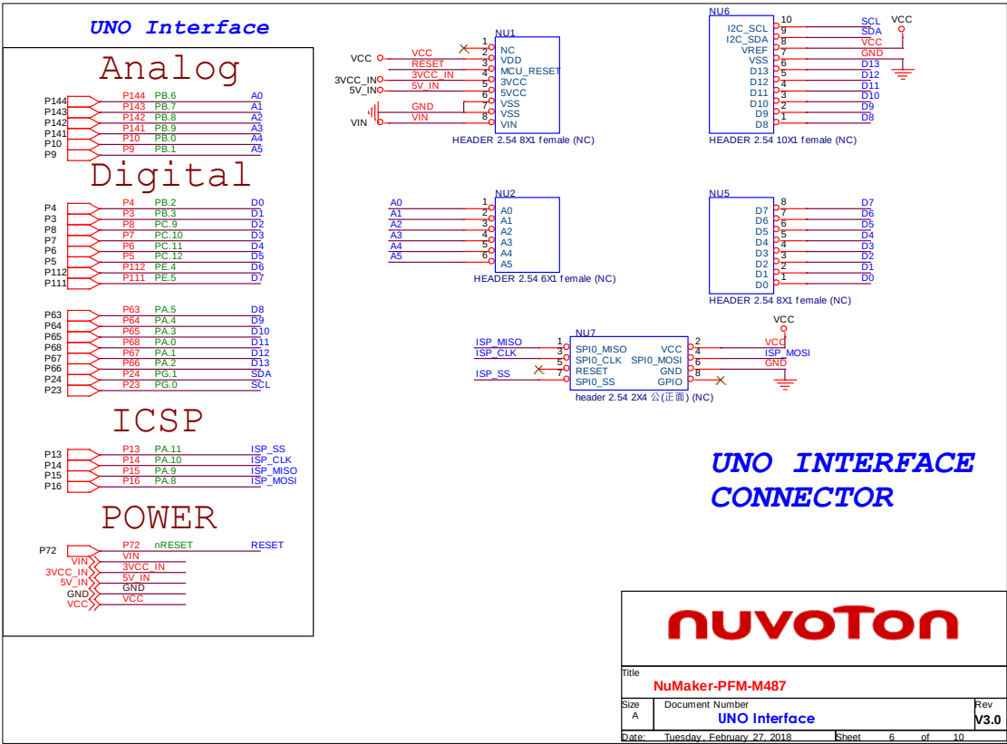
Figure 2-11 Arduino UNO Compatible Interface
