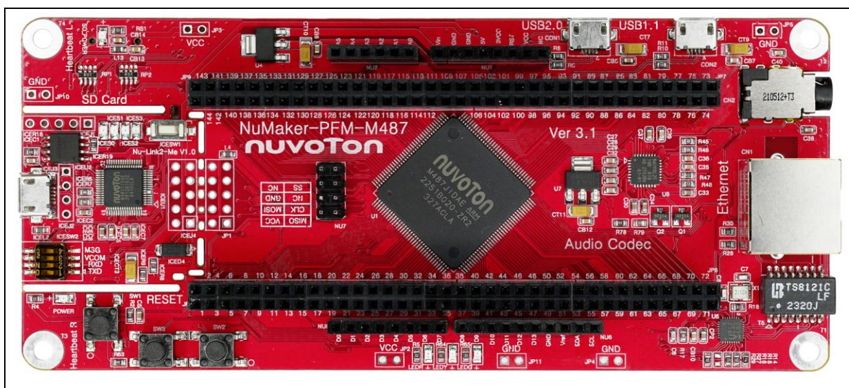
Figure 2-1 NuMaker-PFM-M487 Board
