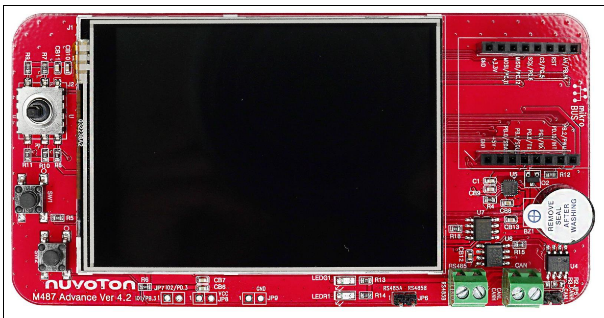
Figure 3-1 NuMaker M487 Advance Board
