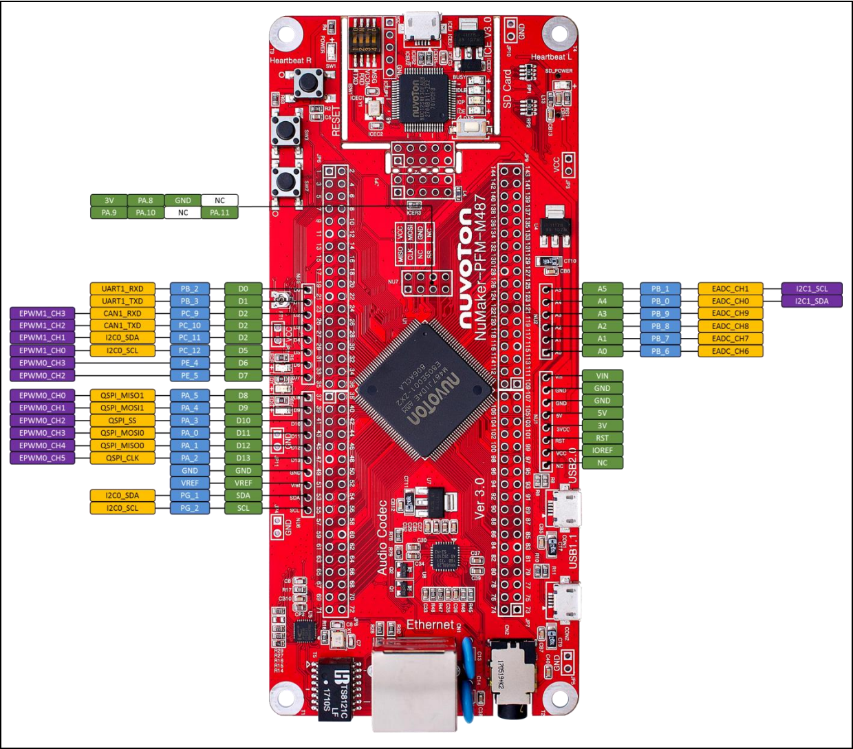
Figure 2-4 Arduino UNO Compatible Interface
