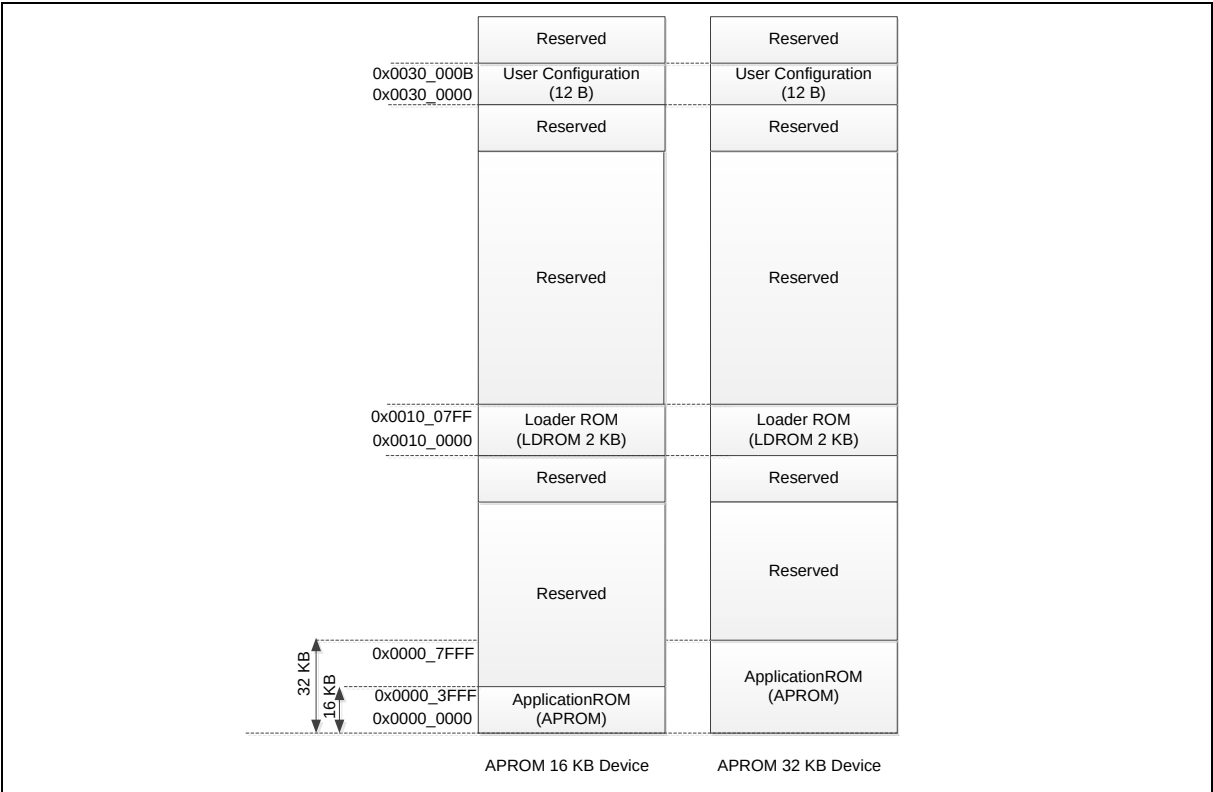
Figure 6.4-3 16/32 Kbytes Flash Memory Map
