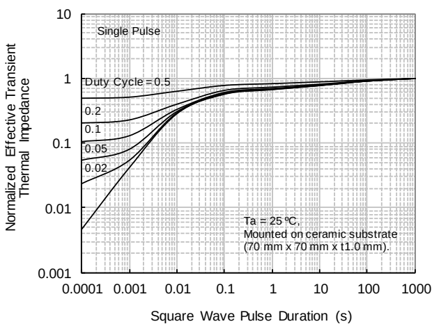
Thermal Response
