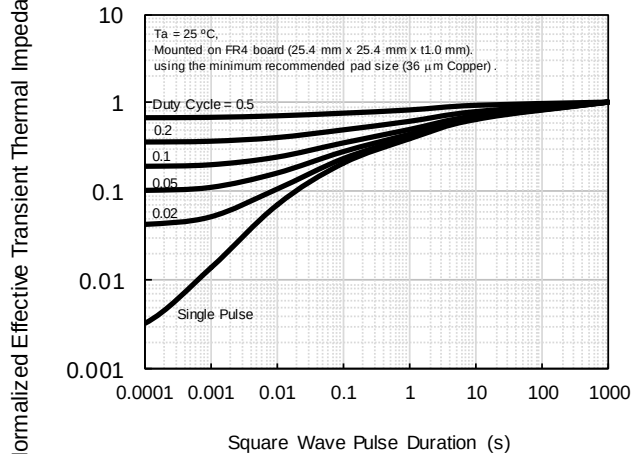
Thermal Response
