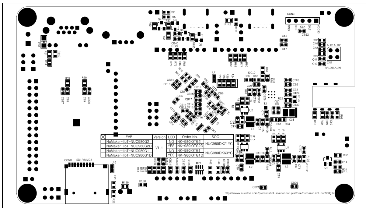
Figure 5-16 Rear Placement
