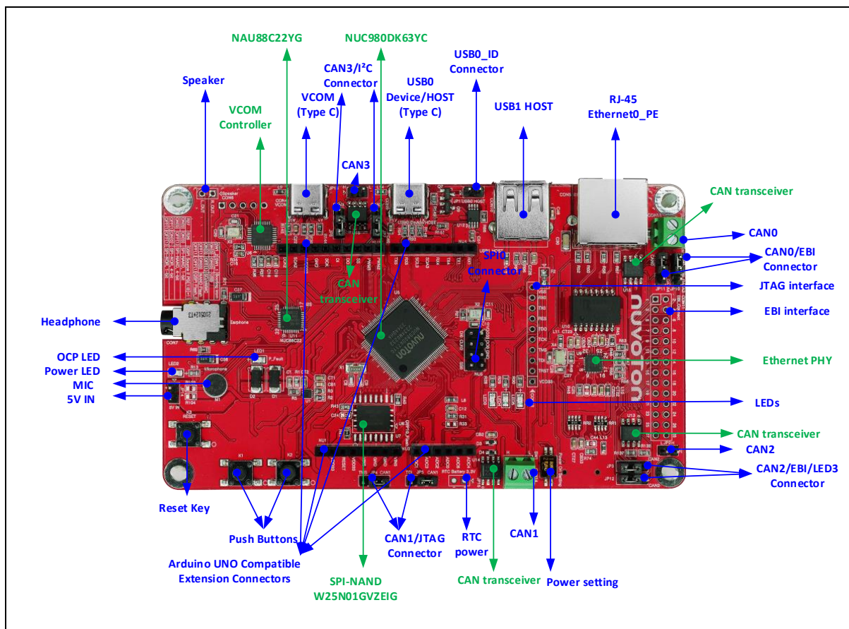
Figure 3-1 Front View of NuMaker-IIoT-NUC980G1
