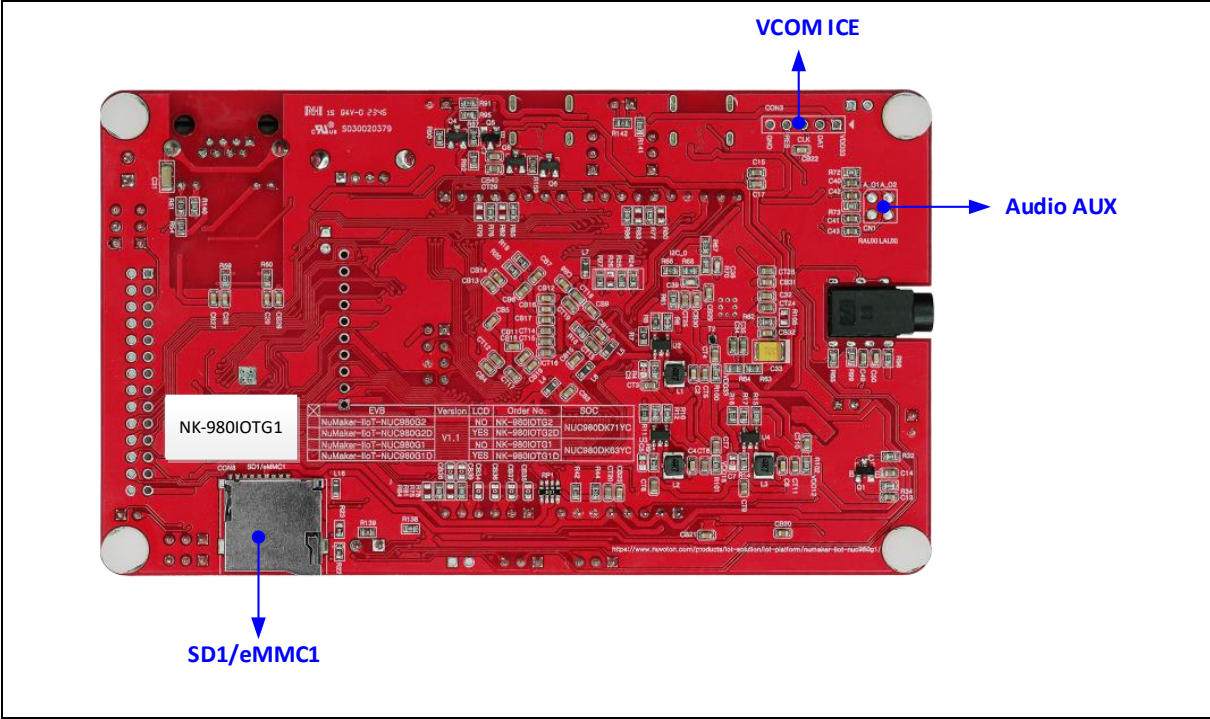
Figure 3-2 Rear View of NuMaker-IIoT-NUC980G1
