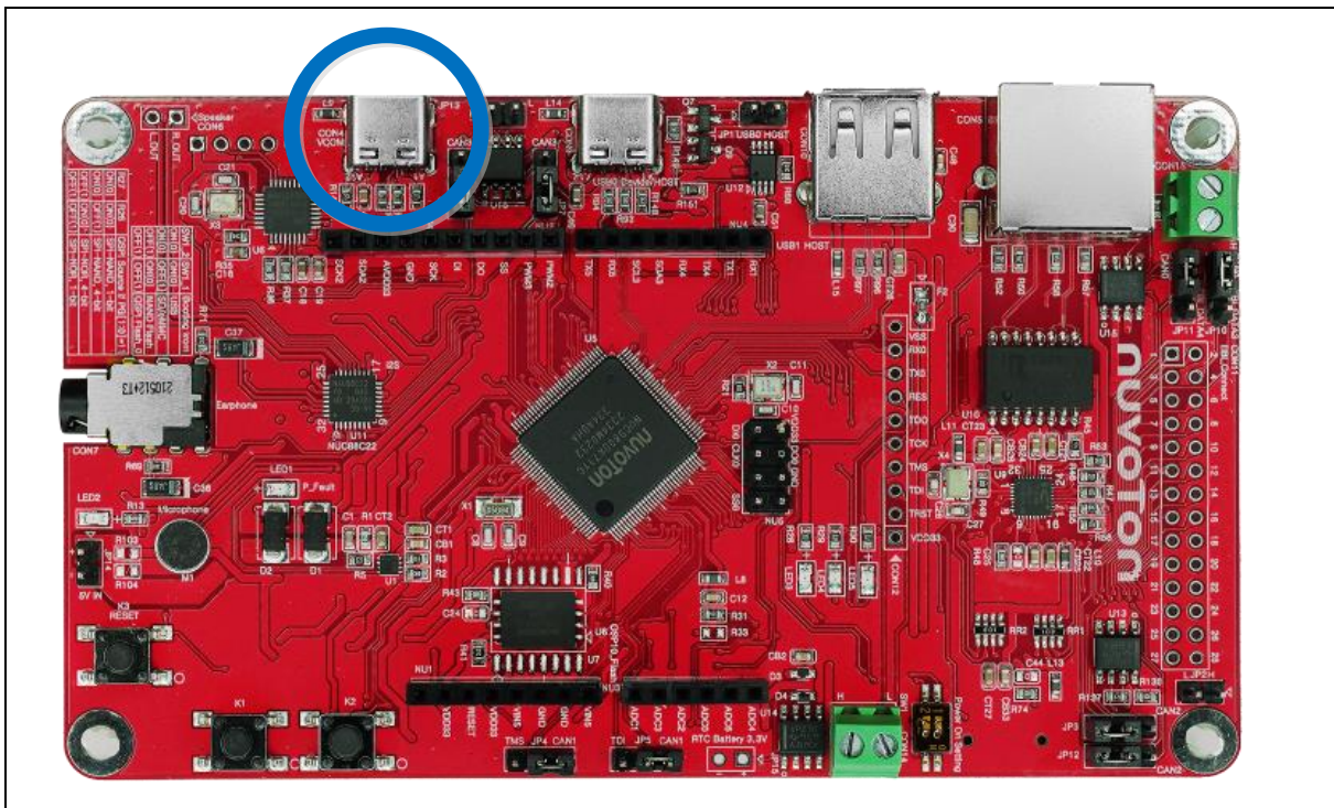
Figure 4-6 USB-Serial Debug Port
