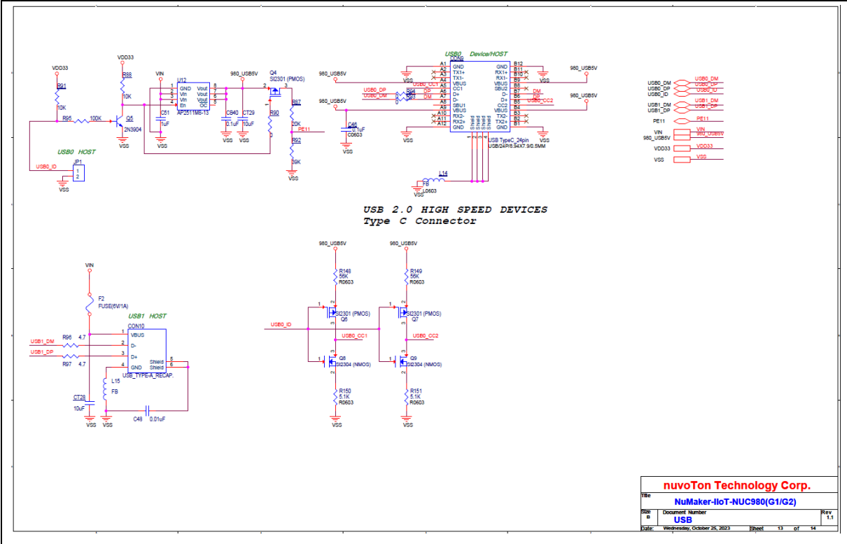
Figure 5-13 USB
