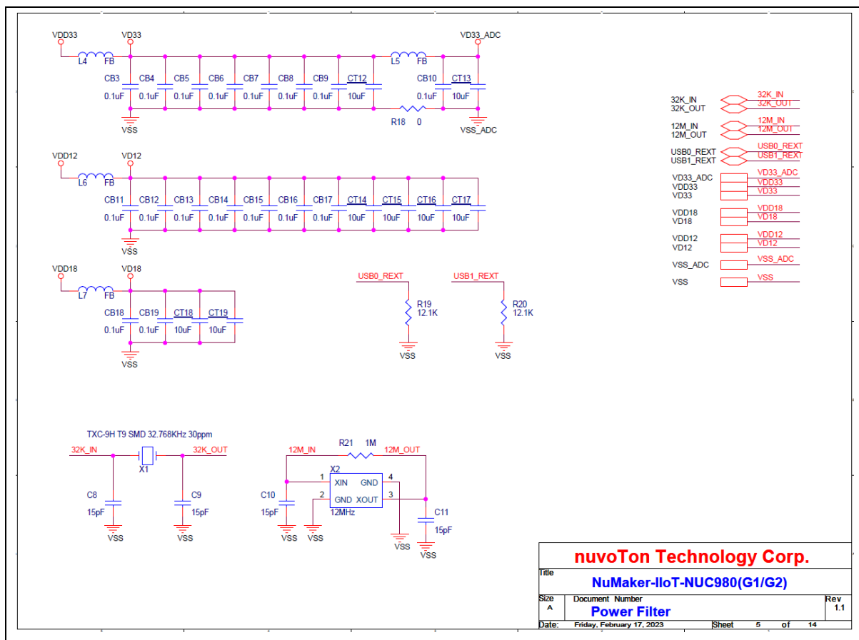
Figure 5-5 Power Filter
