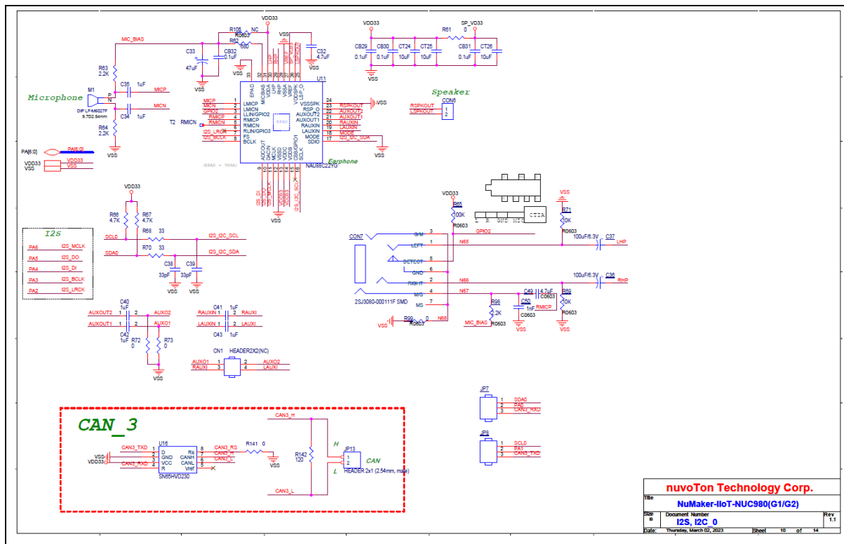
Figure 5-10 Audio Codec and CAN_3
