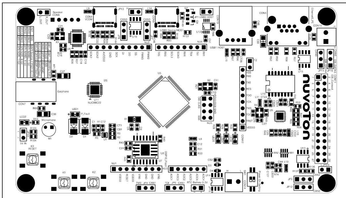
Figure 5-15 Front Placement
