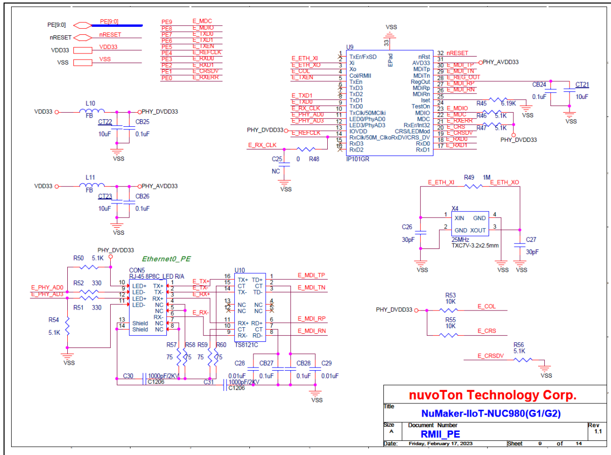
Figure 5-9 RMII_PE
