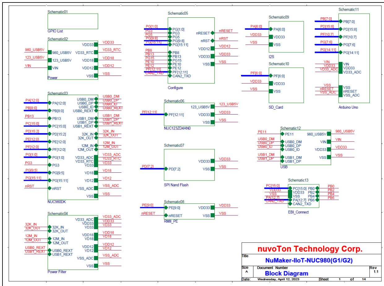
Figure 5-1 NuMaker-IIoT-NUC980G1 Board Block Diagram
