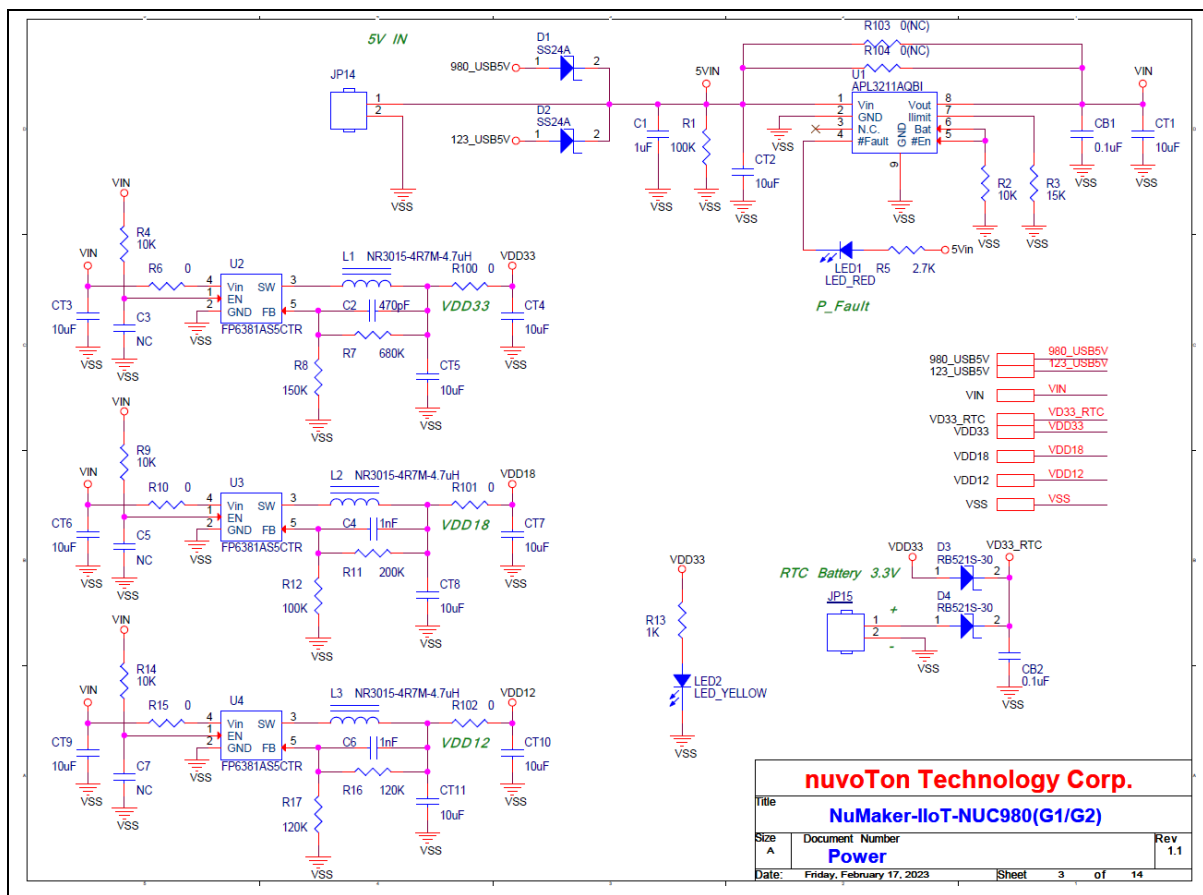
Figure 5-3 Power
