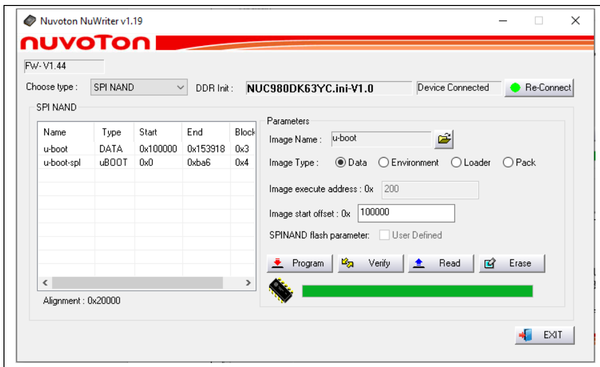
Figure 4-14 Download u-boot to SPI NAND
