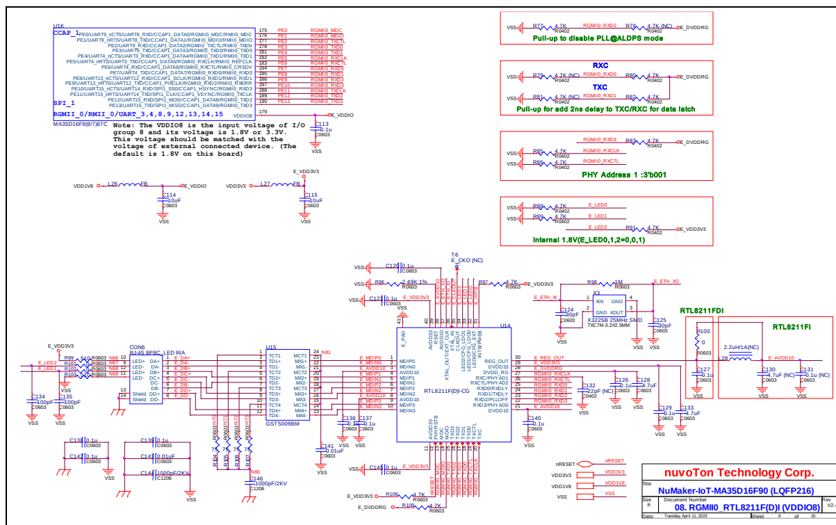
Figure 6-8 RGMII0 PE Schematic
