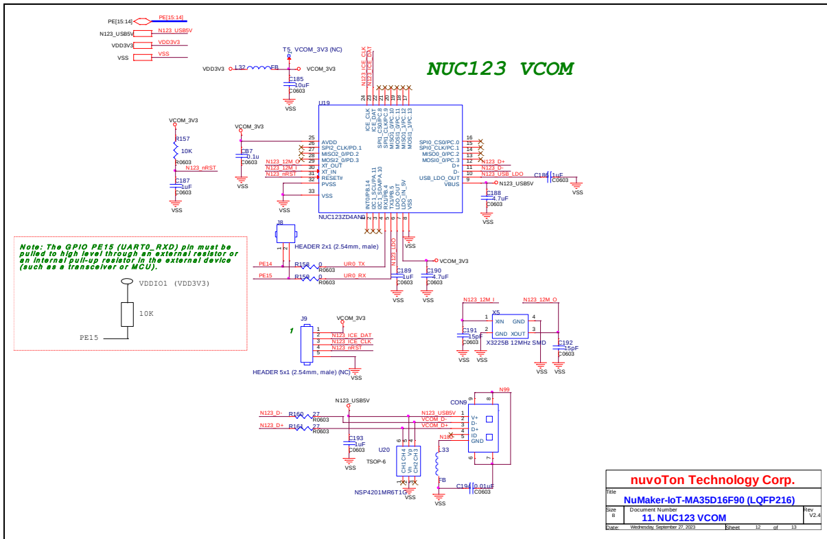
Figure 6-11 NUC123 VCOM Schematic
