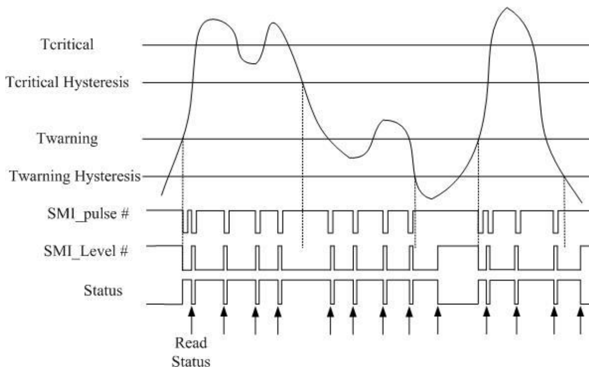
SMI comparator mode
