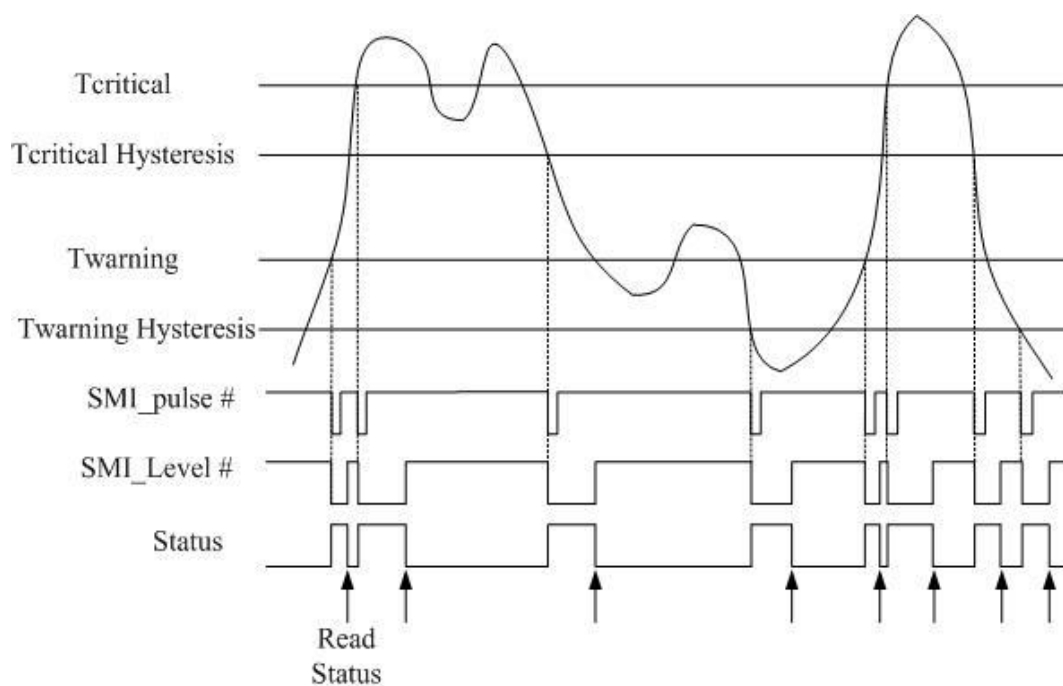
SMI two time mode
