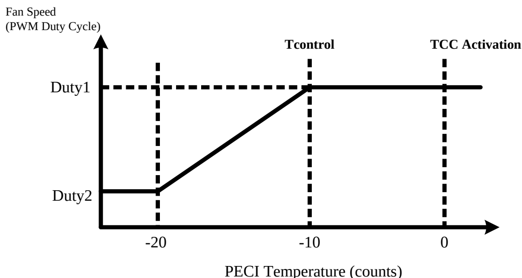
Fig. A PECl Temperature
