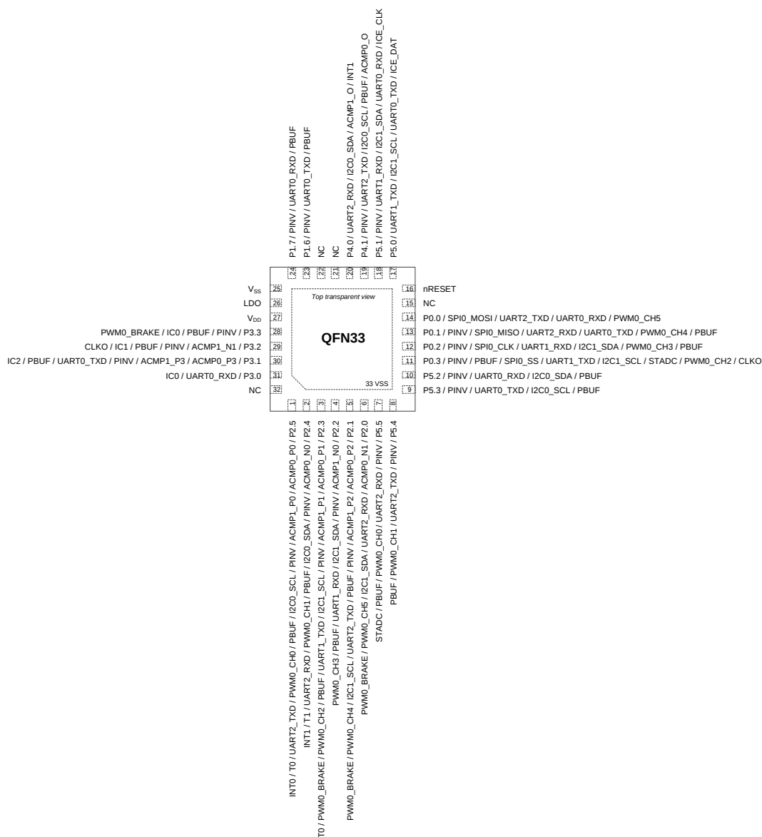
Figure 4.1-2 MUG51TB9AE Multi-Function Pin Assignment
